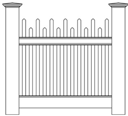
Style 2
