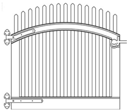
Style G5
