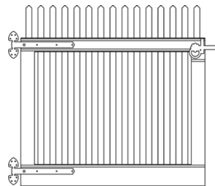
Style G1
