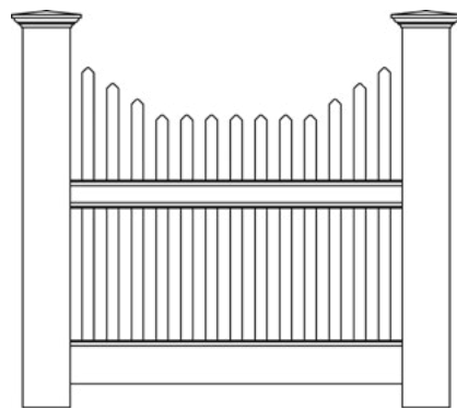
Style 3
