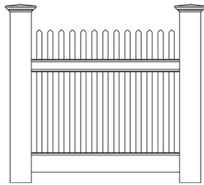
Style 1
