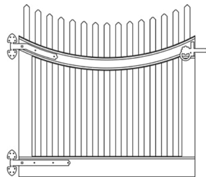
Style G4
