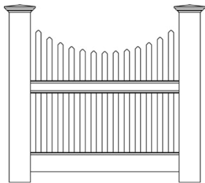
Style 4
